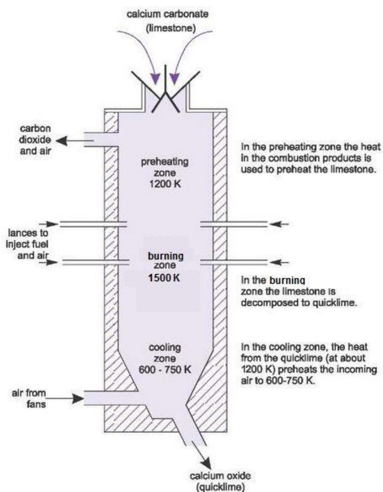
Figure 1: Structure of kiln
